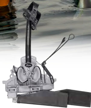
MirageDrive 180 with Kick-Up Fins
