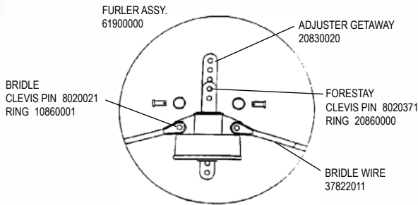
ROLLER FURLER DETAIL
