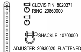
ROLLER FURLER DETAIL
